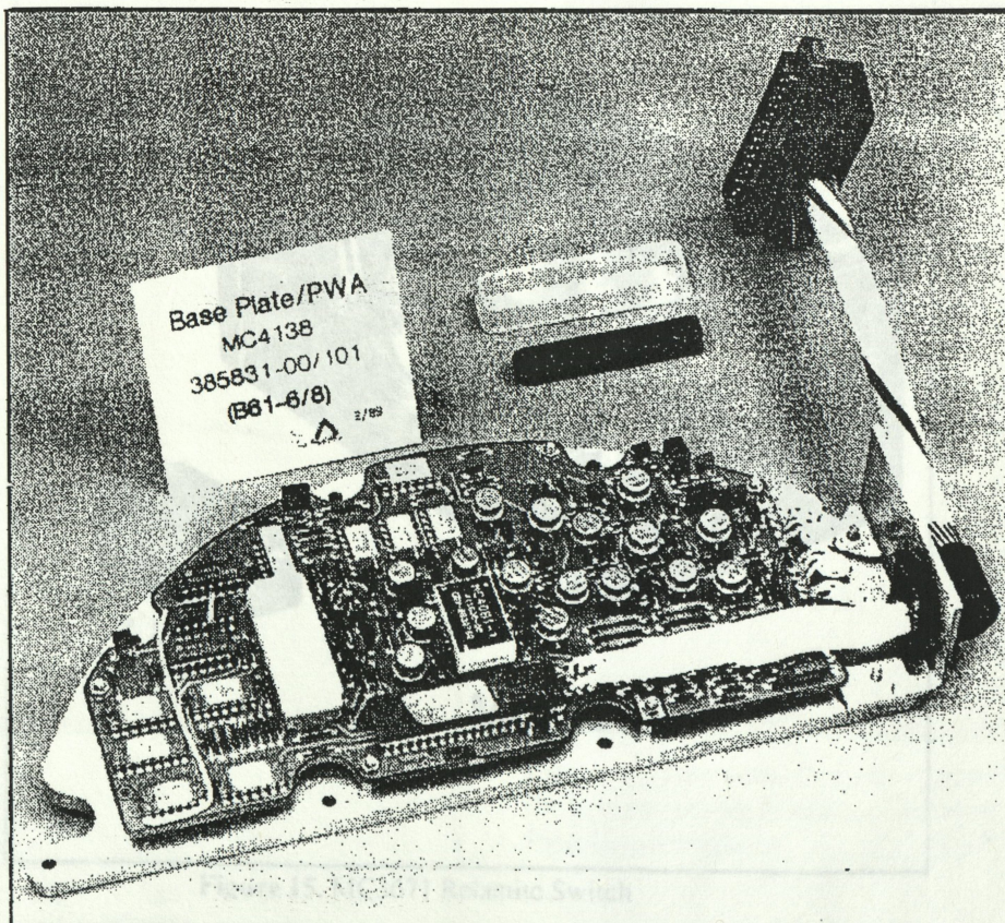
Figure 13. Printed wiring assembly of a single channel of the MC4138 Programmer.
